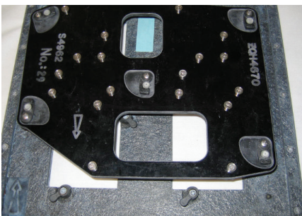
Soldering frames, palettes and masks
